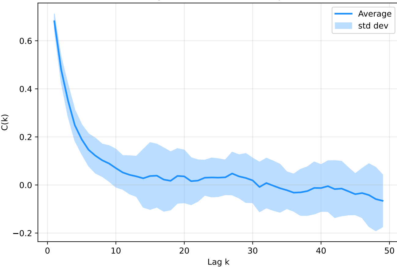
GAP - Average autocorrelation for Experiment 2A
