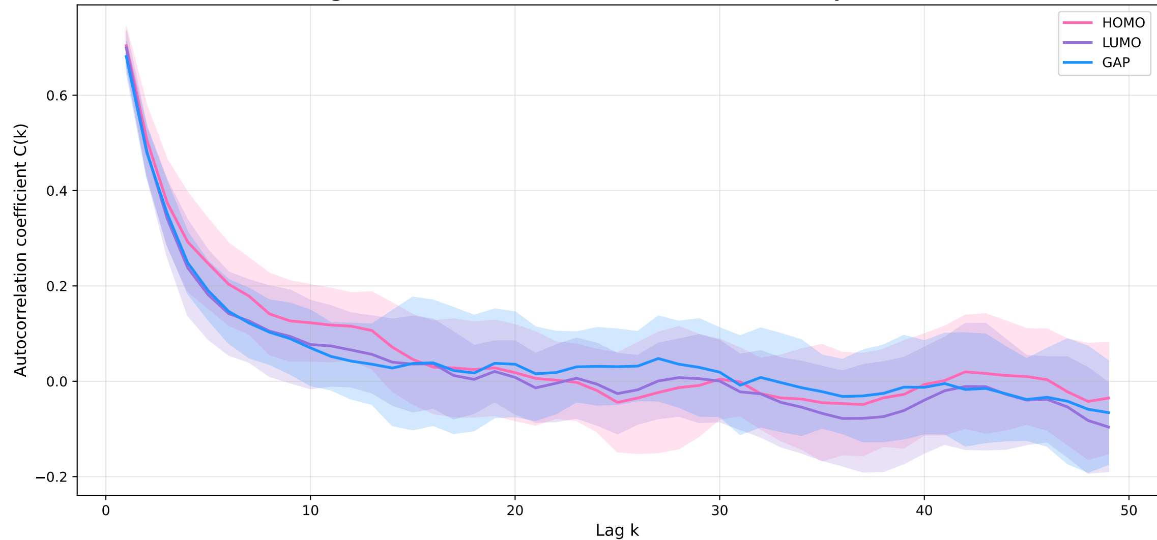
Average autocorrelations (HOMO, LUMO, GAP) for Experiment 2A
