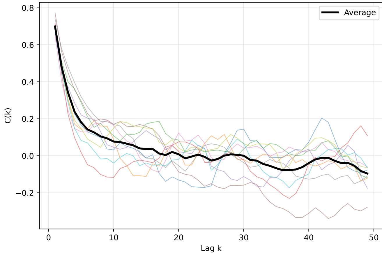
LUMO - All autocorrelation for Experiment 2A
