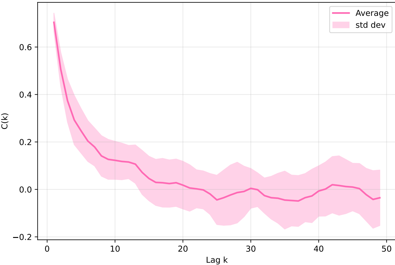
HOMO - Average autocorrelation for Experiment 2A
