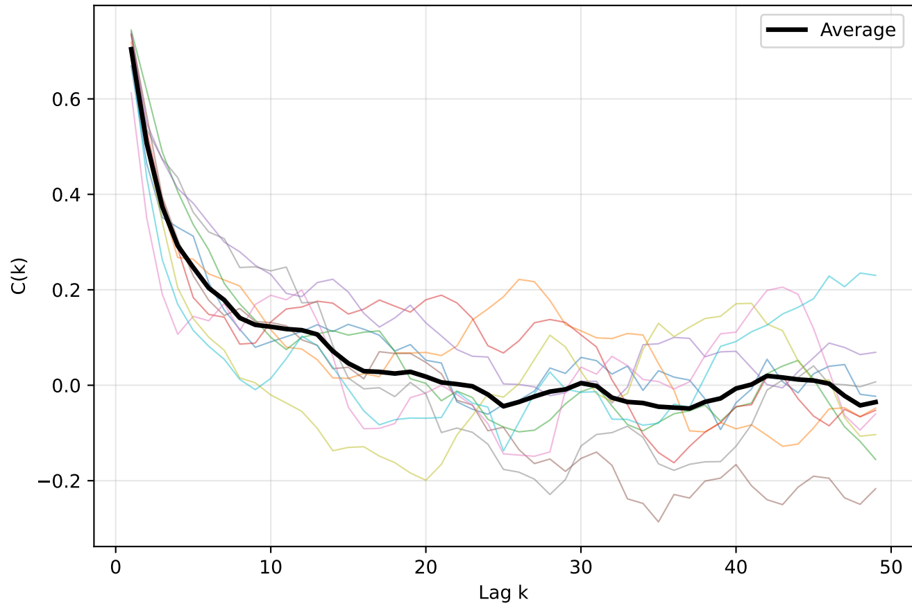
HOMO - All autocorrelation for Experiment 2A
