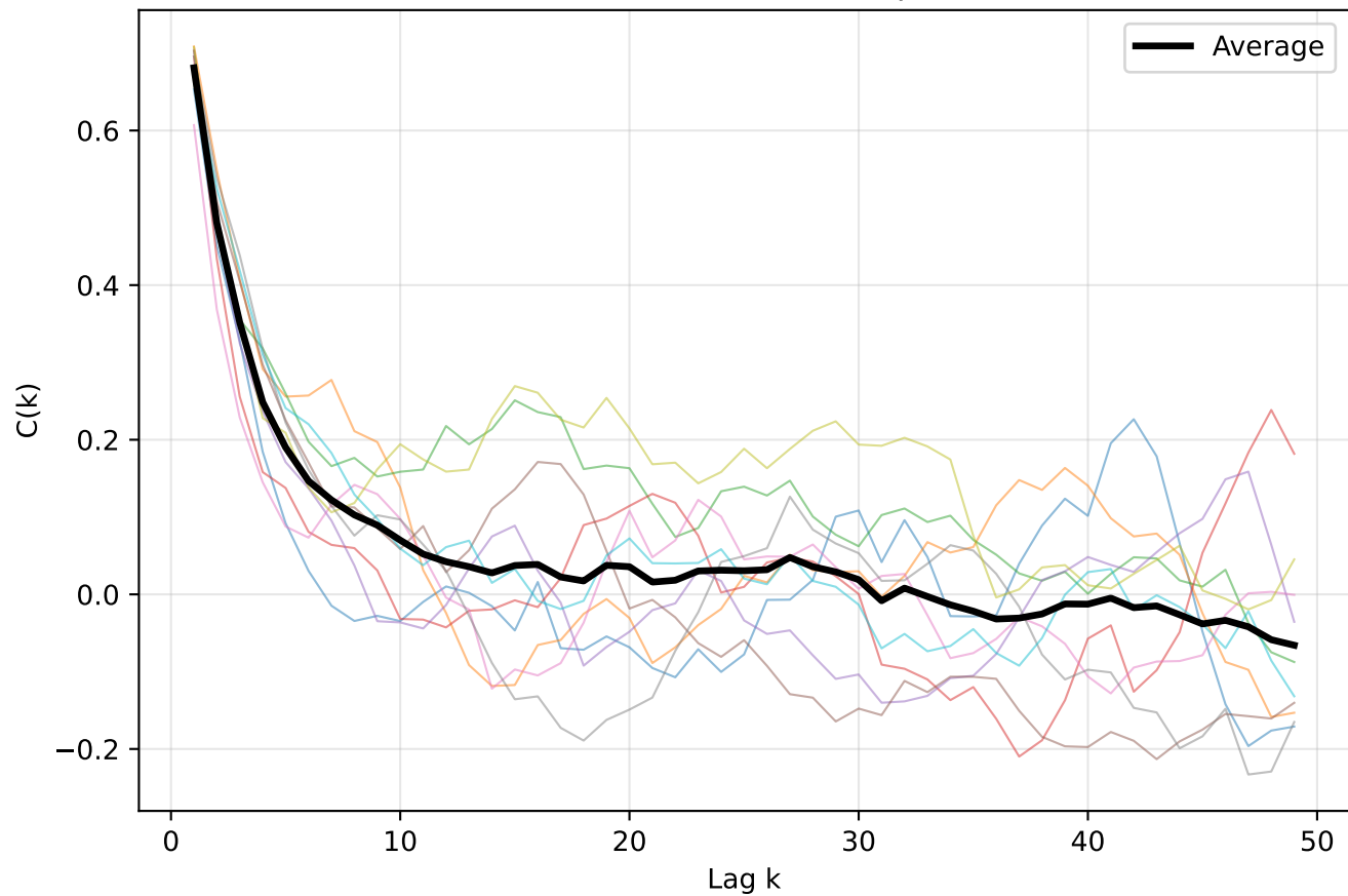
GAP - All autocorrelation for Experiment 2A
