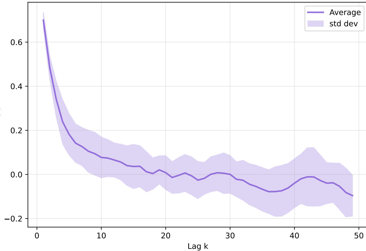
LUMO - Average autocorrelation for Experiment 2A
